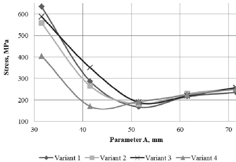
Figure 8. Changing of stresses in the weld root relative to parameter A when B = 20 mm, for four variants.
